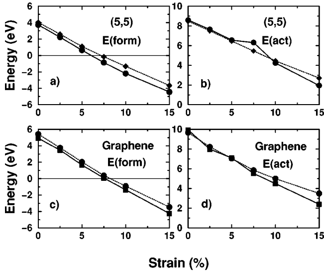
FIG. 3. Comparison between ab initio and tight-binding results for a (5,5) nanotube and a graphene sheet. (a), (c) Formation energies; (b), (d) activation energies. The ab initio results are connected by a solid line, while a dashed line connects the tight-binding results.
