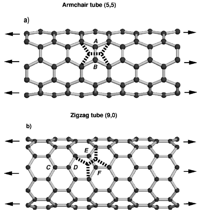
FIG. 1. Bond rotation in strained carbon nanotubes: (a) side view of a (5,5) armchair tube under axial strain: rotating the bond “AB” by 90° forms a (5-7-7-5) defect (dashed lines). (b) Side view of a (9,0) zigzag tube where the bond “EF” is responsible of the formation of the (5-7-7-5) defect (dashed lines). See text.
