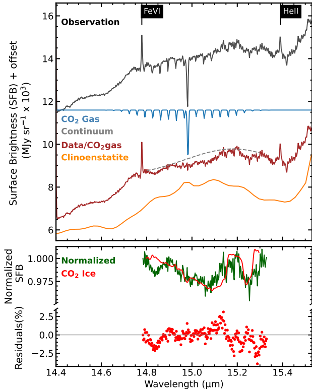
Fig. 1. Detection of CO 2 ice and gas. The overplotted black curve shows the JWST/MIRI spectrum at the position indicated by the dot in Fig. A.1. The uncertainties on the surface brightness are \sim\pm 40 MJy sr -1 . The best-fit gas-phase model ( T_{\text{gas}} = 30 K and \log N = 16.8 cm -2 ) is shown in blue. We divided out this model, resulting in the brown curve. The orange curve shows a single-temperature model for clinoenstatite emission. The dashed gray line shows the continuum we adopted to analyze the ice band. The green curve shows the normalized spectrum using that continuum. The red curve shows a laboratory spectrum for CO 2 ice (CO:CO 2 2:1 ice mixture at 80 K); and the bottom panel shows the residuals between the normalized spectrum (green) and the ice model (red).
