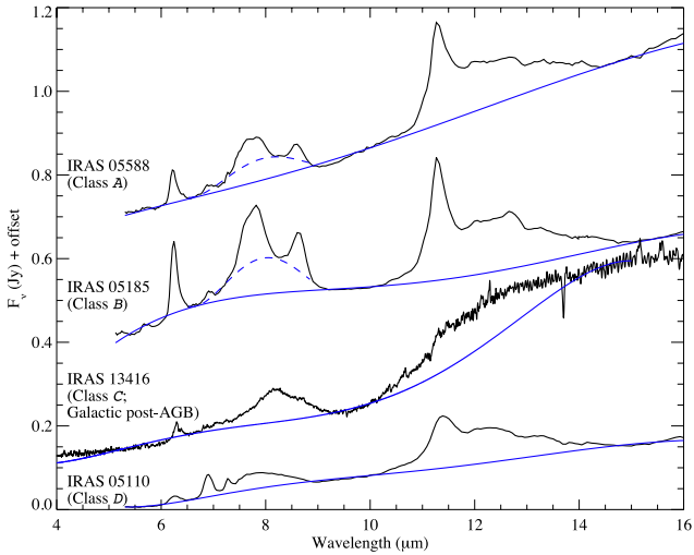
Figure 11. Examples of the continua (blue lines), which were subtracted from the observed spectra, in order to emphasize the intrinsic PAH spectra. The local continua at 6.5–9 \mu\text{m} are indicated by dashed lines.
