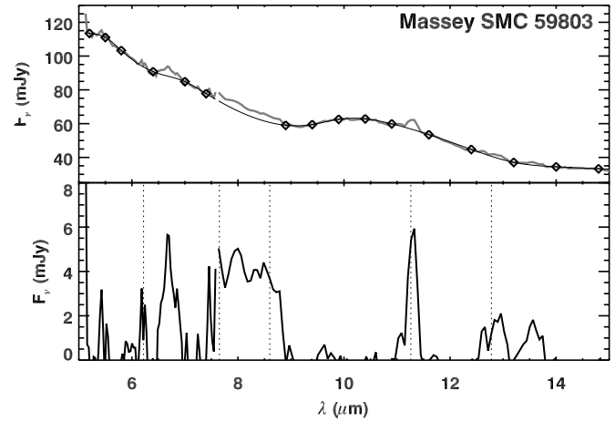
FIG. 24.—Spectrum of Massey SMC 59803 with a fitted spline ( top ), and the residual PAH spectrum ( bottom ). The dashed vertical lines in the bottom panel are at wavelengths of 6.23, 7.70, 8.60, 11.26, and 12.70 \mu\text{m} , the centers of the PAH features in a typical class A PAH spectrum (in the classification system introduced by Peeters et al. 2002).
