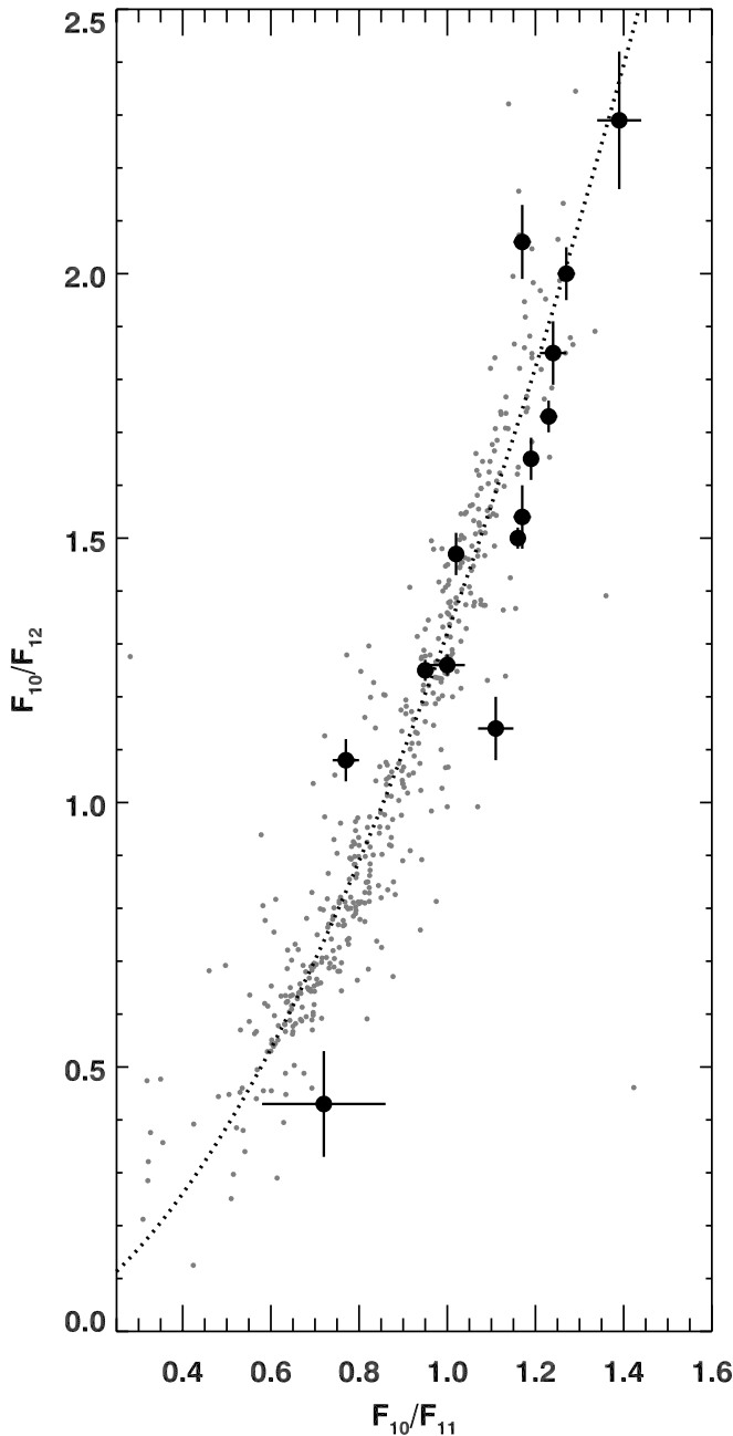
FIG. 11.—Silicate dust sequence. MC_DUST sources are plotted with black filled circles. The smaller gray circles show the distribution of Galactic AGB sources (Sloan & Price 1995, 1998), and the dotted line is a power law: F_{10}/F_{12} = 1.32(F_{10}/F_{11})^{1.77} .
