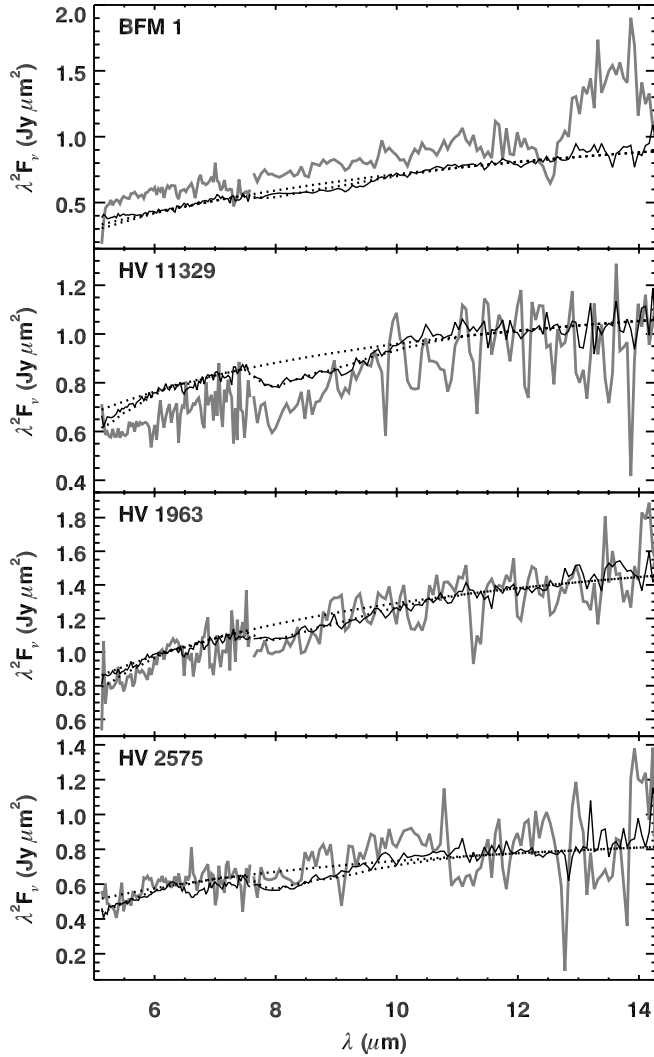
FIG. 7.—Follow-up spectra with longer integration times of four of the MC_DUST targets. The originally observed spectrum appears in light gray, while the new spectrum is in black. The dotted lines are the continuum fitted to the new spectrum and the best-fit absorption spectrum, as in Fig. 3.
