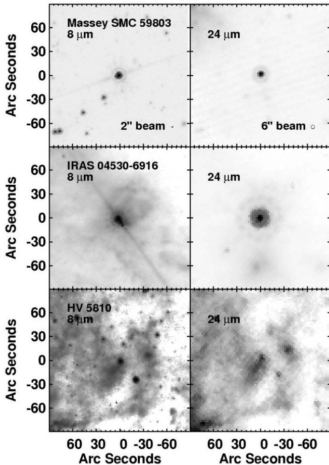
FIG. 23.—The 8 and 24 \mu\text{m} fields of the three PAH sources shown in Figs. 8 and 22. The images of Massey SMC 59803 and IRAS 04530 are plotted on a logarithmic scale, while HV 5810 is plotted on a linear scale. Massey SMC 59803 is an isolated supergiant, but the other two sources are associated with extended emission.
