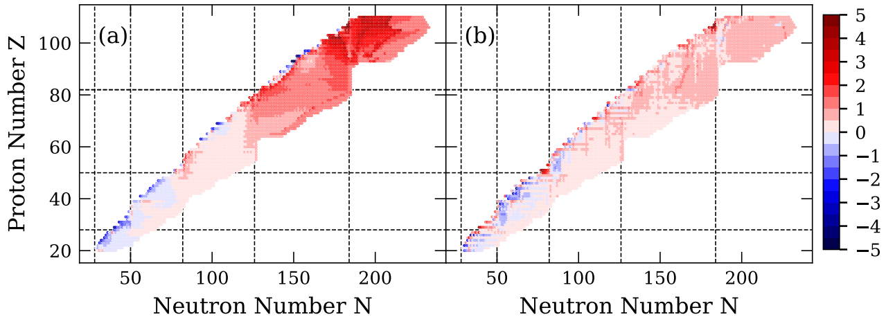
FIG. 7. Log of the ratio of our half-lives to those of a) Ref. [12] and b) Ref. [11].
