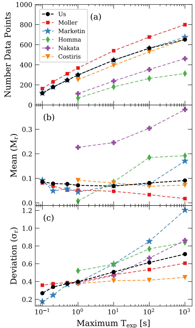
FIG. 6. Comparison of error-evaluation parameters among results of Refs. [12] (Marketin), [11] (Möller), [46] (Costiris), [10] (Nakata), and [17] (Homma).
