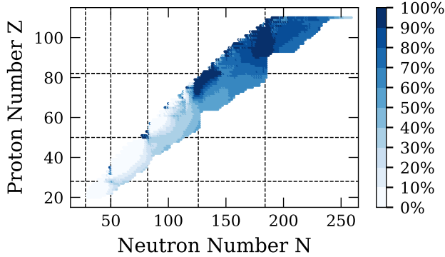
FIG. 4. First-forbidden contribution to the rates.
