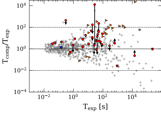
FIG. 3. Same as panel b) of Fig. 1 but compared with 2019 ENSDF data. Only odd nuclei are shown.
