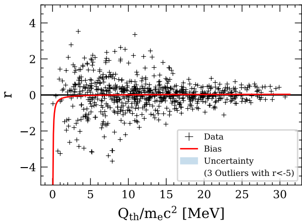
FIG. 5. Bayesian fit to the bias function and one- and two-standard-deviation bands.
