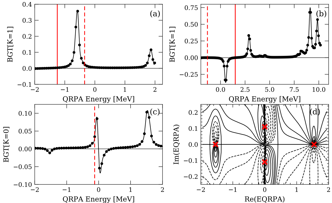
FIG. 2. Examples in which contour integration fails. The dashed vertical line indicates the left bound of the contour from Eq. (18), while the solid line indicates the adjusted bound required to correct the rate. Panels a) and b) show the Gamow-Teller ( K=1 ) strength function for ^{63}\text{Co} and ^{53}\text{Sc} , respectively. Panel c) illustrates an imaginary pole in the response function of ^{173}\text{Er} , and d) shows the response in the full complex plane, indicating poles near \omega = \pm 0.1i .
