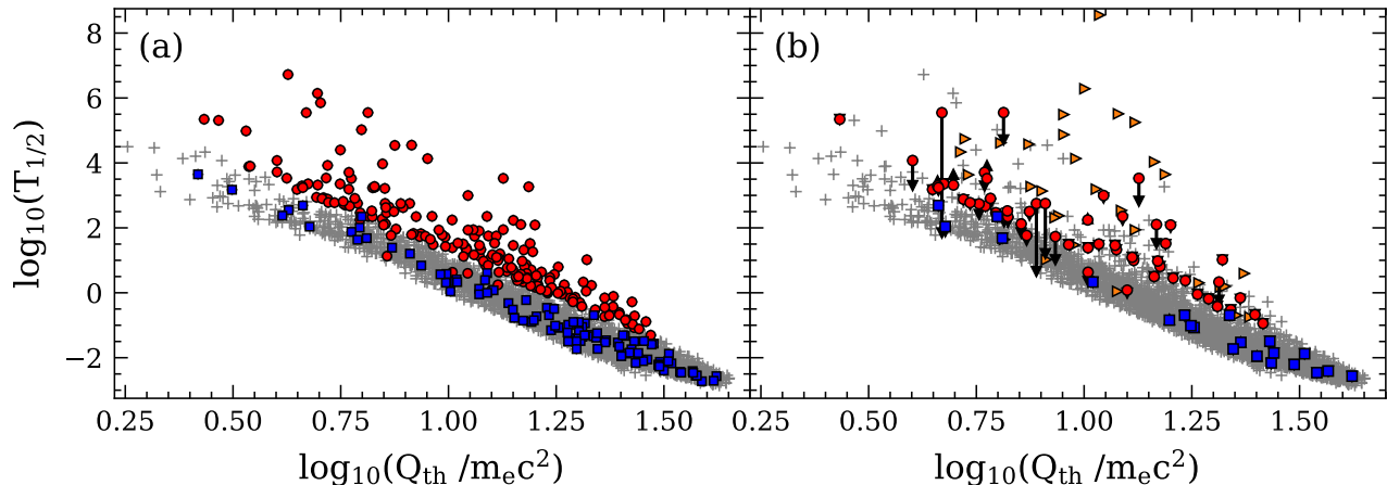
FIG. 1. Corrections of half-lives in odd nuclei. Half-lives for which we calculate strength functions are in panel a). Red circles are for the 224 suspicious nuclei and blue squares for the 100 nuclei from the random sample. Panel b) shows half-lives that are corrected as described in the main text, with corrected values indicated by black arrowheads. Orange triangles are corrected versions of originally negative half-lives.
