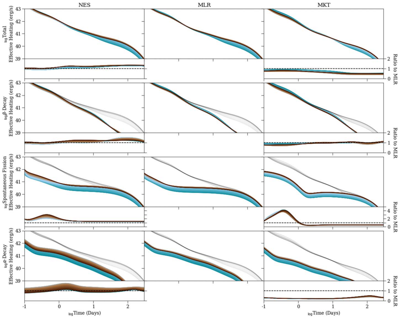
Figure 8. Range of effective heating rate predictions using the FRDM2012 mass model with 50/50 fission product yields when composite- Y_c trajectories are considered. From left to right, the beta-decay description used is NES , MLR , MKT . The color scheme corresponds to that shown in Figure 2. As in Figure 3, we replicate the total heating curves shown in the top row in the bottom three rows as light gray lines for easier comparison.
