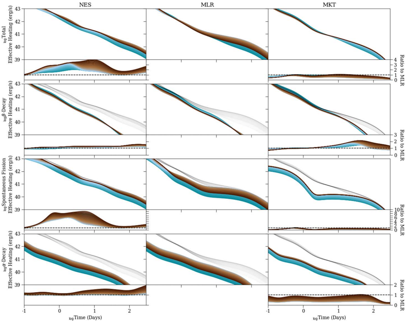
Figure 9. Range of effective heating rate predictions using the HFB22 mass model when composite- Y_c trajectories are considered with 50/50 fission product yields. From left to right, the beta-decay description used is NES , MLR , MKT . The color scheme corresponds to that shown in Figure 2. As in Figure 3, we replicate the total heating curves shown in the top row in the bottom three rows as light gray lines for easier comparison.
