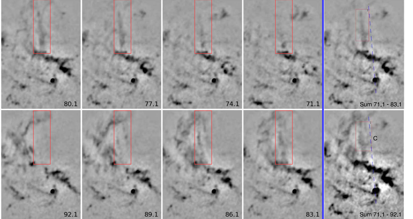
Figure 8. Inverse grayscale image over 1.6 \times 2.3 \text{ arcmin}^2 of ALMA CS ( J = 2 - 1 ) channels, and their sums in the rightmost column; velocity in \text{km s}^{-1} relative to the LSR. The region plotted is similar to that in Figure 5(d). Continuum emission has not been subtracted but is only noticeable at Sgr A* (black dot) and in the minispiral. The proposed jet impact to the north, Anomaly C, is delineated by the red box to show how it shifts from parallel strands starting at bottom left to center filled in the top row. The dashed projected jet axis adjacent to the fainter western strand is drawn near the right side within the box. The rightmost column sums emission over the velocities indicated.
