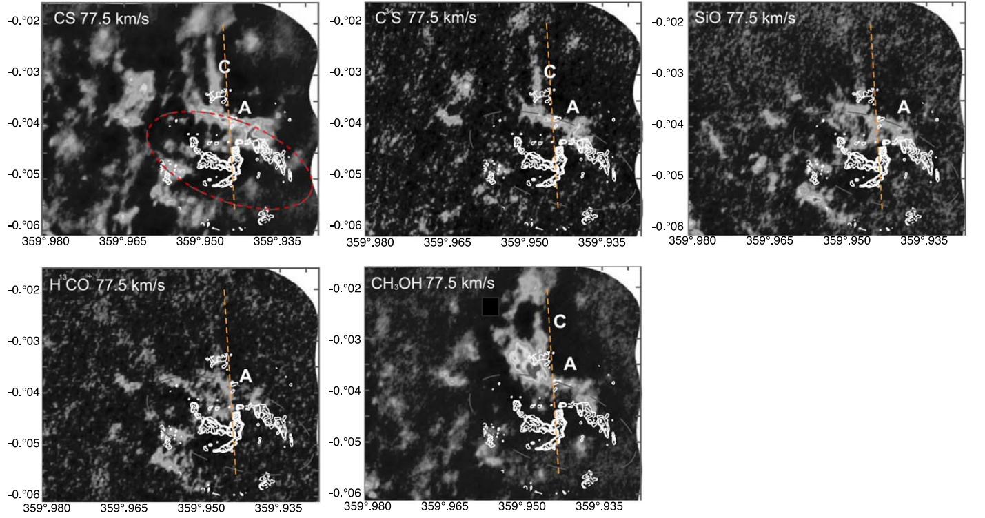
Figure 7. ALMA LSR +77.5 \text{ km s}^{-1} channel in diagnostic lines (based on parts of Figures 3–6 of T18) after continuum subtraction. The lines show that Anomaly C has 10^3 (T_{\text{ex}}/200 \text{ K}) \mathcal{M}_{\odot}^{\text{N}} of weakly shocked molecular gas at \lesssim 10^4 \text{ cm}^{-3} . The CND is the dashed ellipse, and the nuclear minispiral within it is shown as white 100 GHz continuum contours. The dashed line extrapolates the southern jet—Sgr A* axis to the north; it lies slightly west of Anomaly C.
