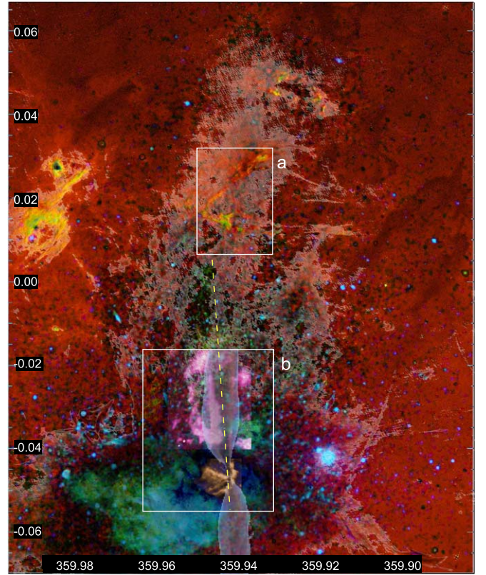
Figure 1. This region at the GC with degree labels shows X-rays, energetic electrons, and molecular gas overlaid on Paschen \alpha from the Hubble Space Telescope (HST) in rust color. The last, shown log-scaled, brightens through orange to yellow especially in the minispiral around Sgr A* in the lower quarter of box (b) that delineates Figure 5 panels (b)+(d). The northern X-ray lobe delineated by Chandra in green (2–4 keV) and blue (4.5–8 keV, mostly within the CND and at many compact sources) is spanned by radio continuum filaments (ragged gray–white overlay) mapped by the JVLA (shown alone in Figure 2(e)). Within box (b) in pink is the redshifted ALMA CS emission discussed in Section 3.3. In translucent overlay is one of our smaller-scale 3D simulations launched along the dashed yellow jet axis. The larger-scale simulation is compared to data in Figures 3 and 31. Box (a) spans Figure 11.
